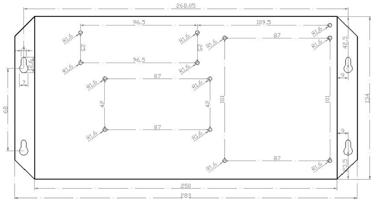
MR-218DW Rear view
